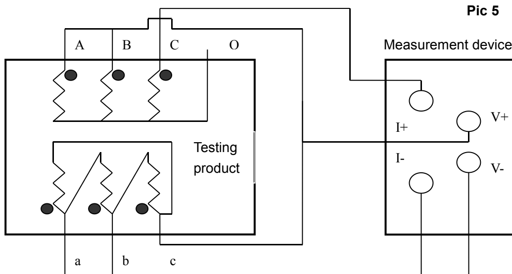
Picture 3, 4, 5 respectively measure low voltage R_{ac} , R_{ba} , R_{cb} connection
