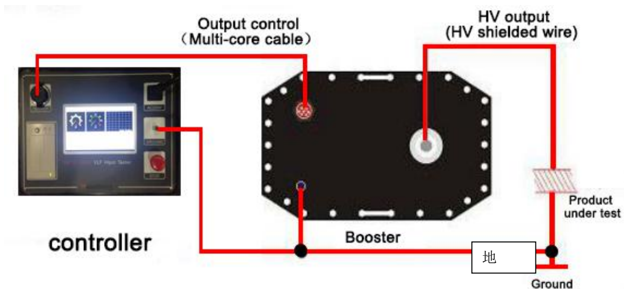
Figure 3 wiring diagram
